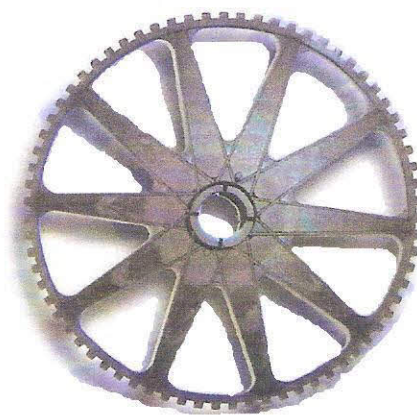
EDB013 Somet - SM92 D.255 x D.30 - Z=71
